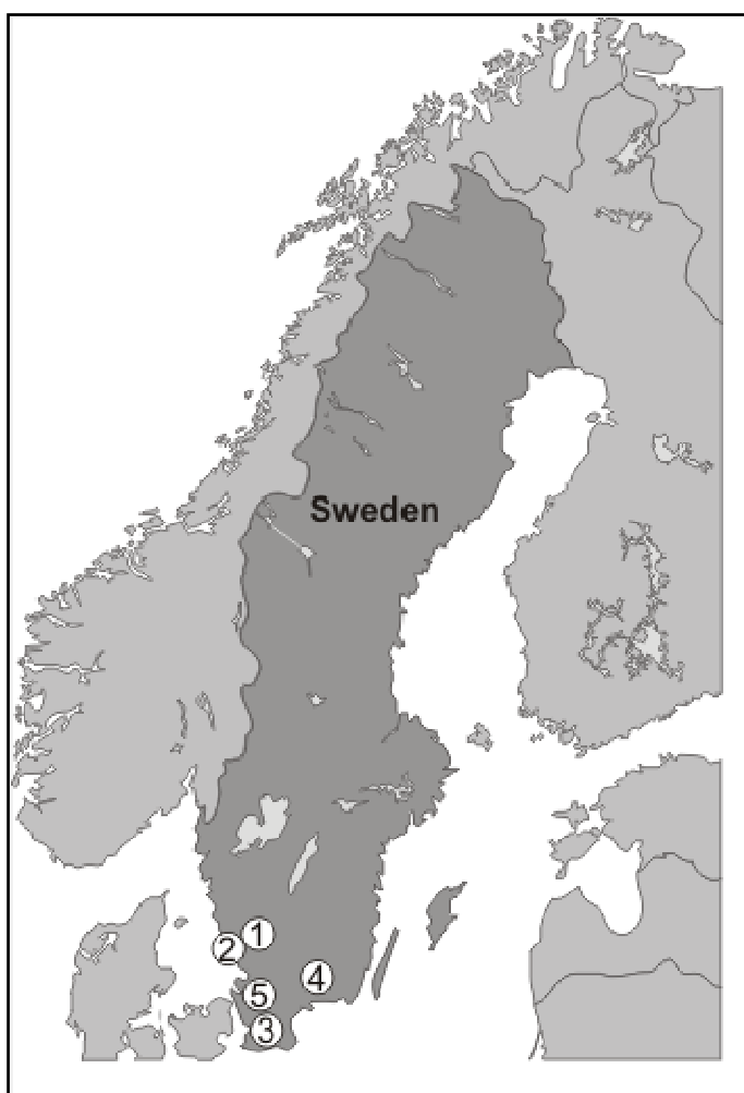
Figure 1: Study sites in southern Sweden
