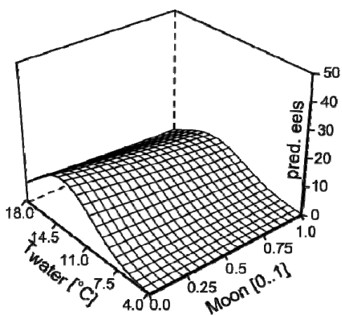
Figure 19: Model surface for Håstad Mölla model daily spring 2013
