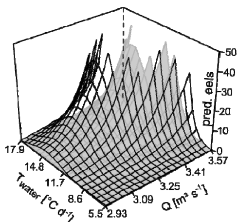
Figure 20: Model surface for Håstad Mölla model daily autumn 2012
