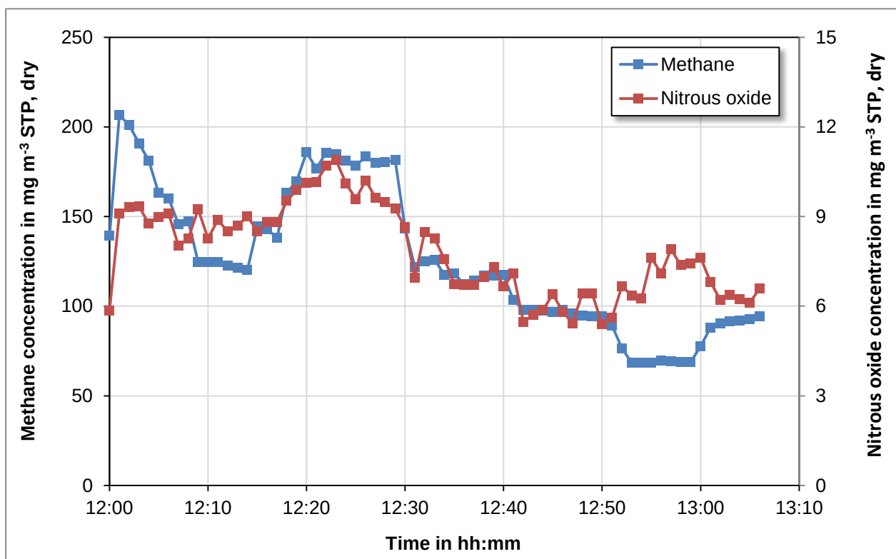
Figure 20: Mass concentration of methane and nitrous oxide from the biofilter
