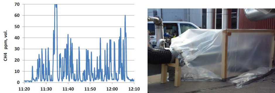
Figure 13. DGC results and sampling set-up at homogenization tank – hole.
