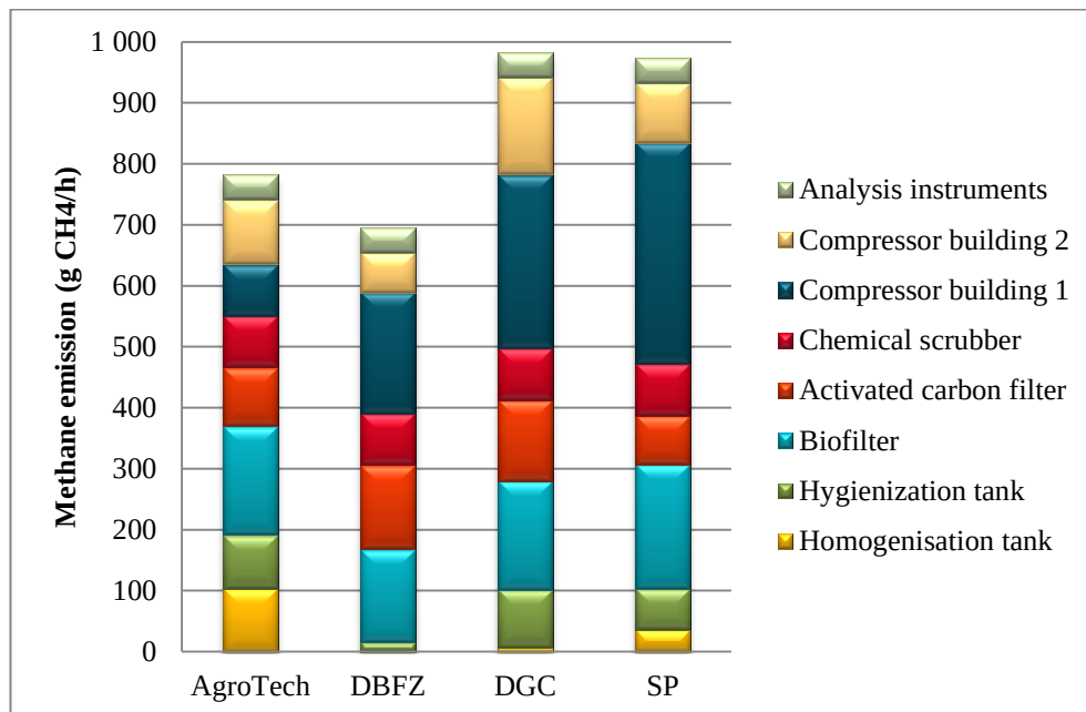
Figure 20. Comparison of estimated/hypothetical values for emission sources of low magnitude.
