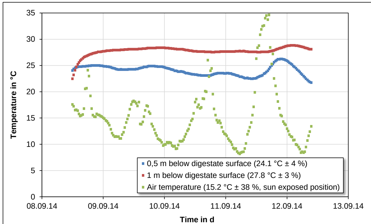
Figure 15: Digestate and air temperature during the investigation period (declared values are average ± standard deviation)
