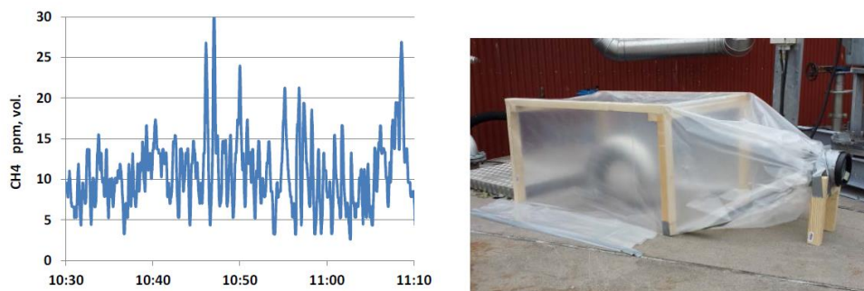
Figure 14. DGC results and sampling set-up at homogenization tank – pipe.
