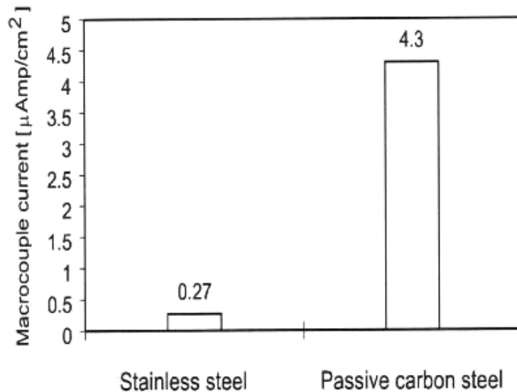
Figure 6 Macrocouple current for stainless steel and passive carbon steel.
