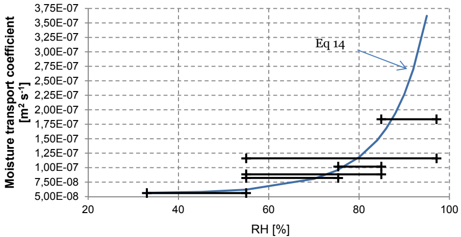
Figure 22. Average measured moisture transport coefficient, at 20 °C, for the Ringhals 4 concrete specimens. The average values were based on the B, C and D measurements, shown in Figure 16. The blue lines correspond to the simulated results using Eq. 14.
