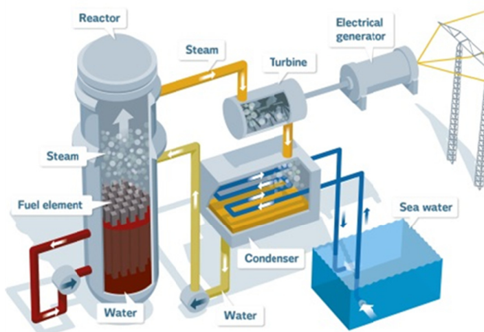
Figure 5. Reactor design and basic function of a BWR. In a BWR, steam is produced directly in the reactor and later used to propel the turbine in one primary circuit. (Figure owned by Vattenfall AB, published with their permission)
