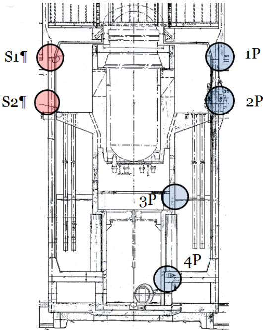
Figure 29. Section of Forsmark 2 with a schematic location of measurement zones. Zones 1P, 2P, S1, and S2 were located in the inner containment wall, and zones 3P and 4P in the wall separating the lower drywell and wetwell.
