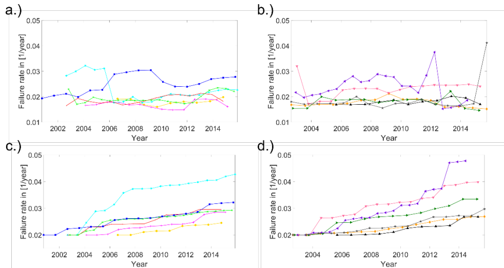
Figure 12: Estimated individual failure rates with suggested risk functions over the time period 2002 to 2015. a.) Individual failure rates for transformers 1-6 with a positive linear risk function for measurement 1, 2, and 4, a negative linear for measurement 3, and the non linear risk function for measurement 5. b.) Individual failure rates for transformers 7-12 with a positive linear risk function for measurement 1, 2, and 4, a negative linear for measurement 3, and the non linear risk function for measurement 5. c.) Individual failure rates for transformers 1-6 calculated with the cumulative risk function for all measurements. d.) Individual failure rates for transformers 7-12 calculated with the cumulative risk function for all measurements.
