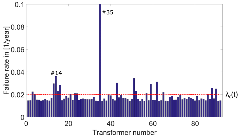
Figure 9: Computed individual failure rates for a population of 92 units with actual failure occurrence for component number 14 and 35
