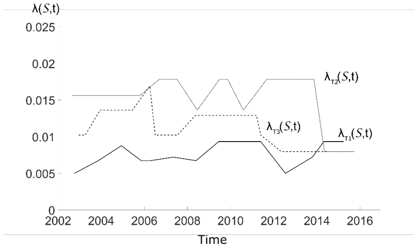
Figure 7: Computed failure rates for three transmission power transformers rated greater 25 MVA based on a health index score presented in [77]
