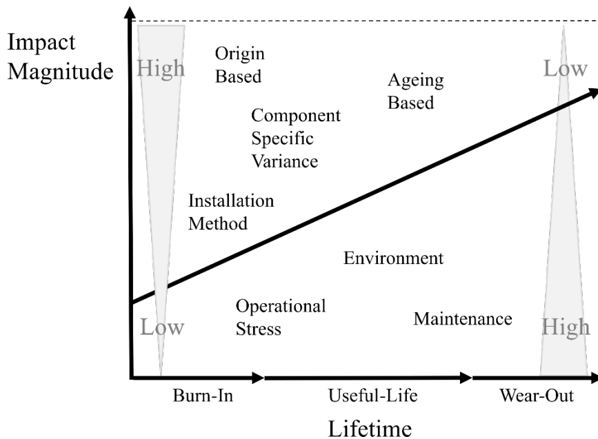
Figure 4: Abstract illustration of the Impact Magnitude of static and dynamic factors on a component's condition development and failure rate over time based on [27]
