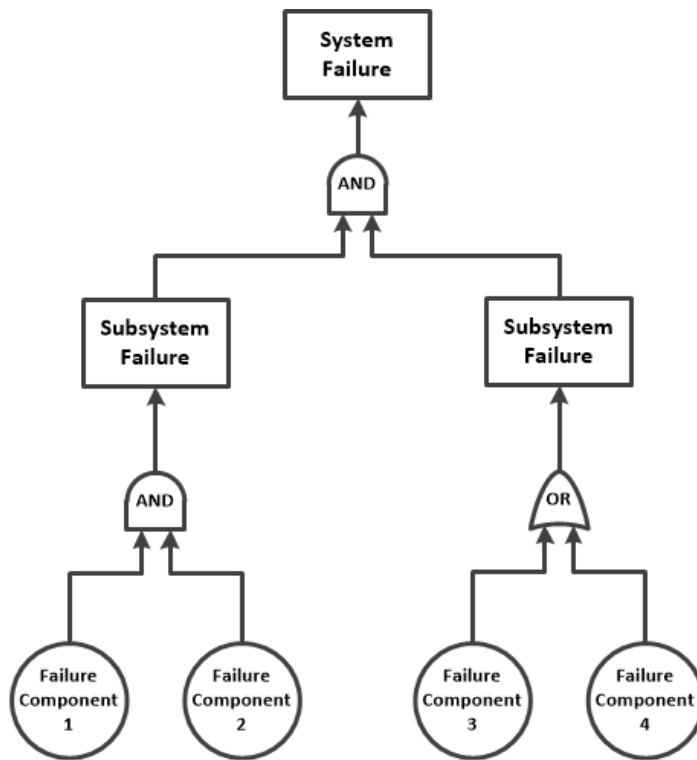
Figure 2: Simplified relationship between component and system reliability.
