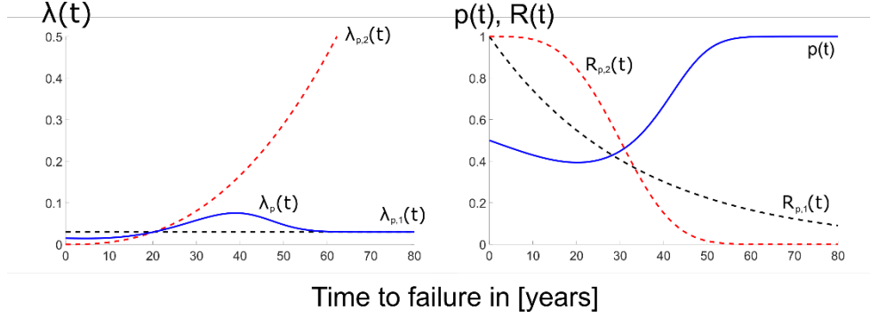
Figure 3: The left part of the figure depicts the population failure rate which is observed as the result of two different subpopulations with \lambda_{p,1}(t)=0.03 and \lambda_{p,2}(t)=0.105 * (0.03 * t)^{3.5-1} for subpopulation 1 and 2, respectively. The right part of the figure shows the survival functions of both subpopulations plus the relative share p(t) of the subpopulations over time.
