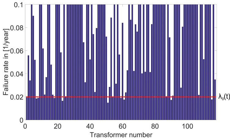
Figure 10: Computed individual failure rates for 117 units with actual failure occurrence based on the published data in [83]
