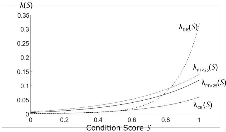
Figure 6: Empirical component failure rate functions based on a condition score for power transformers rated greater 25 MVA \lambda_{PT>25}(S) and smaller 25 MVA \lambda_{PT<25}(S) , disconnectors \lambda_{DIS}(S) , and CB \lambda_{CB}(S) which are presented in [20]
