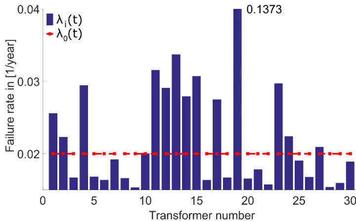
Figure 11: Individual failure rates for transformers 1-30 with the initial average failure rate of 0.02 and a confidence interval of 95%
