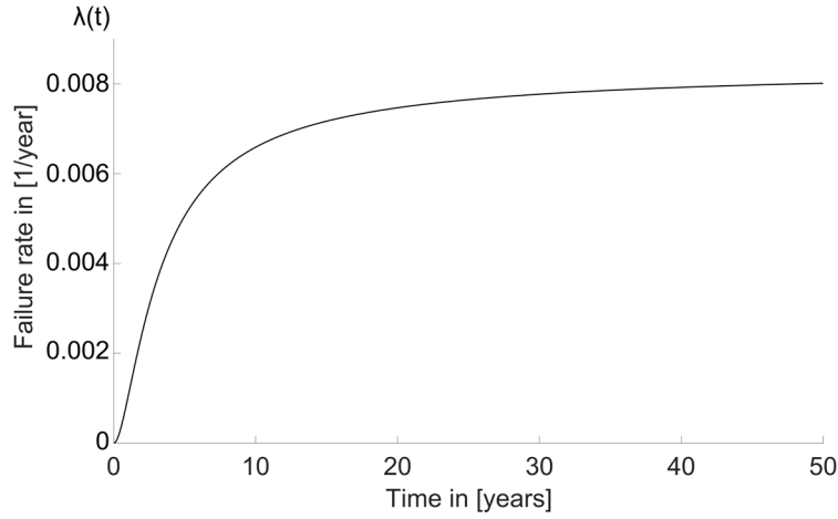
Figure 5: Estimated failure rate based on HMM and dissolved gas analysis data [71]
