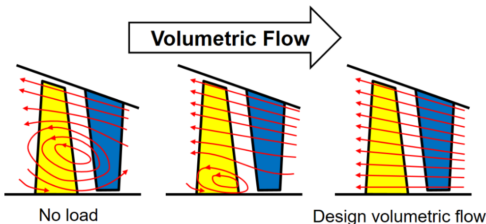
Figur 8-10. Turn-up/ventilation
