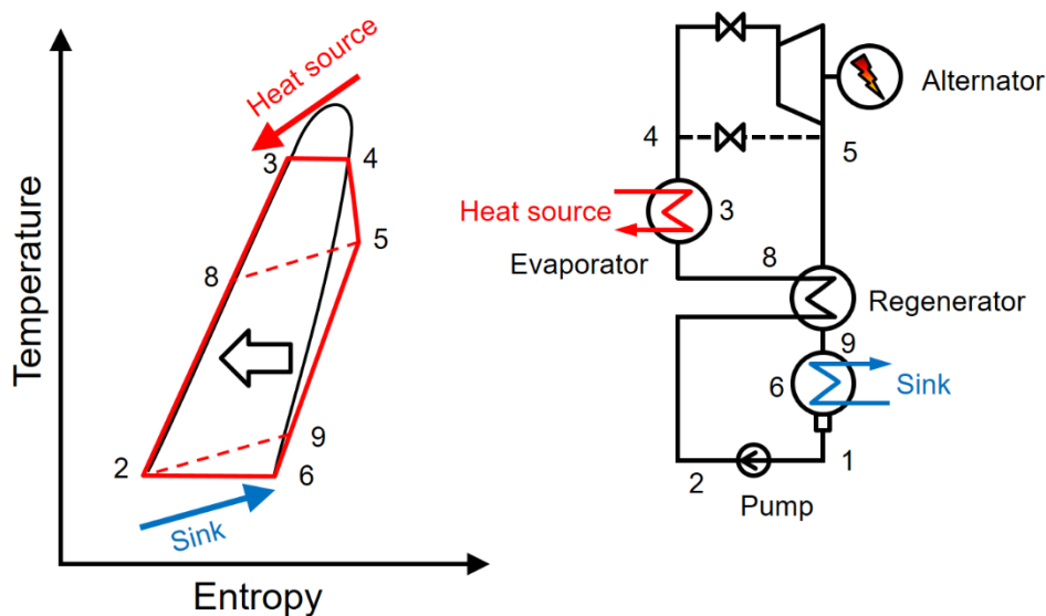
Figur 8-1 ORC-process
