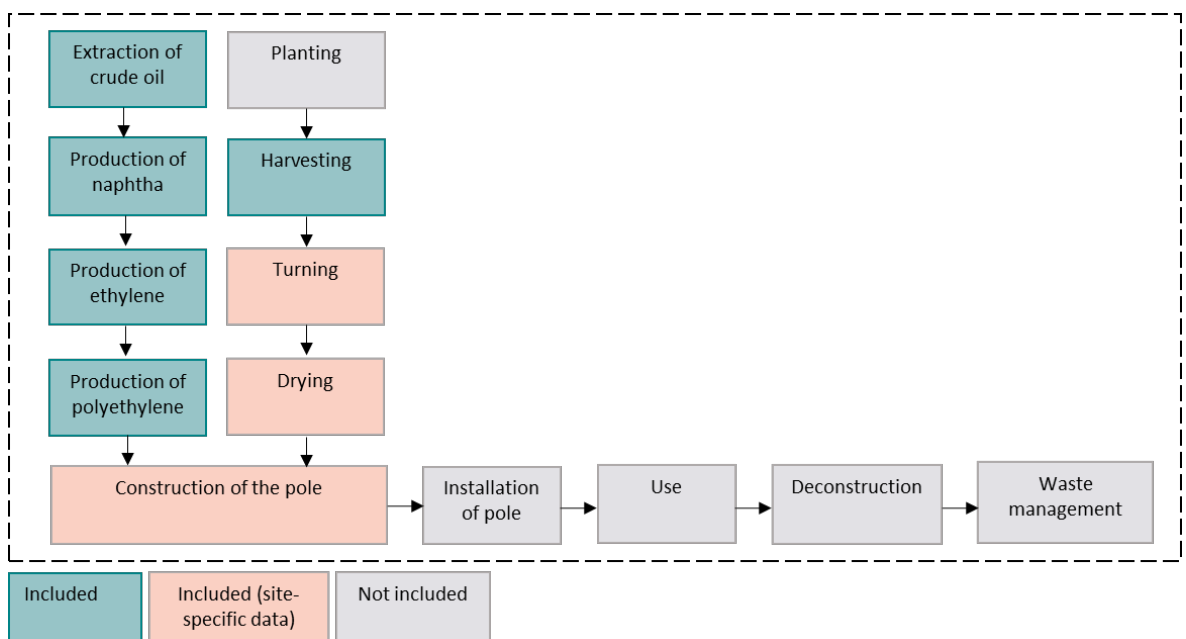
Figure 3 - Overview of the life cycle of the wood pole encapsulated with plastic. The green boxes are the processes included in the assessment, the pink boxes are the process with site-specific data and included the assessment, while the grey boxes are the processes not included.
