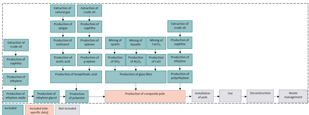
Figure 2 - Overview of the life cycle of the composite pole. The green boxes are the processes included in the assessment, the pink boxes are the process with site-specific data and included the assessment, while the grey boxes are the processes not included.
