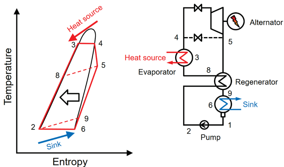
Figur 9-1 ORC-process
