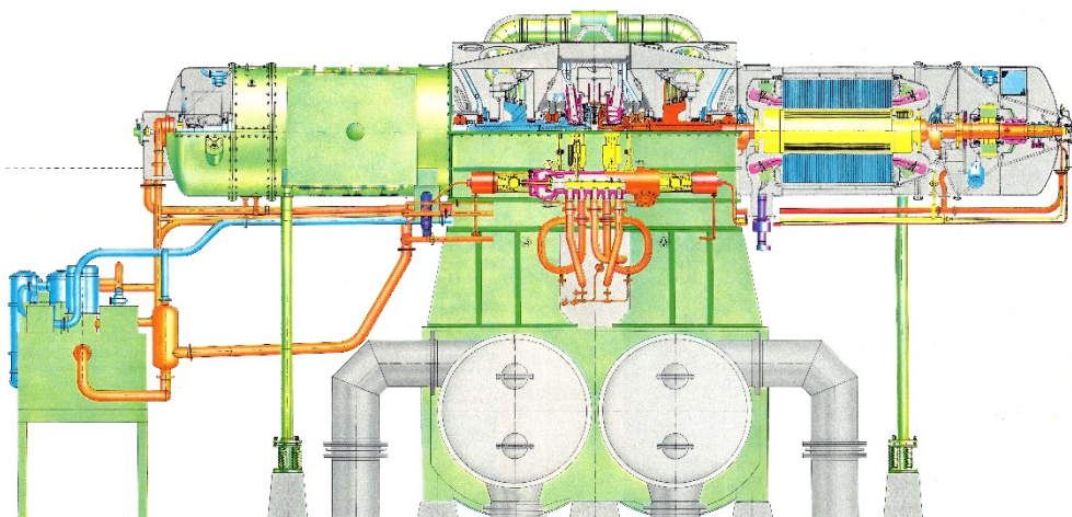
Figur 1-2. Stal-Laval DURAX (radial/axial)
