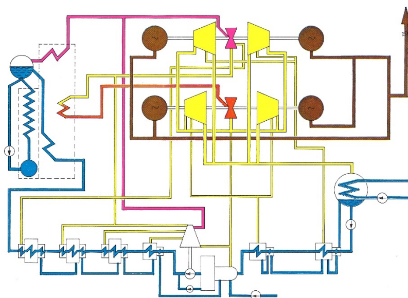
Figur 1-4. Stal-Laval DURAX processschema
