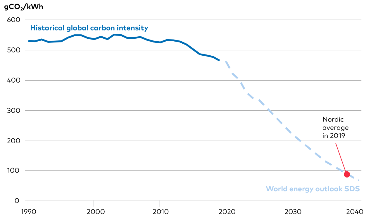
Figure 1.3. Global CO 2 intensity of electricity generation and Nordic Average.
