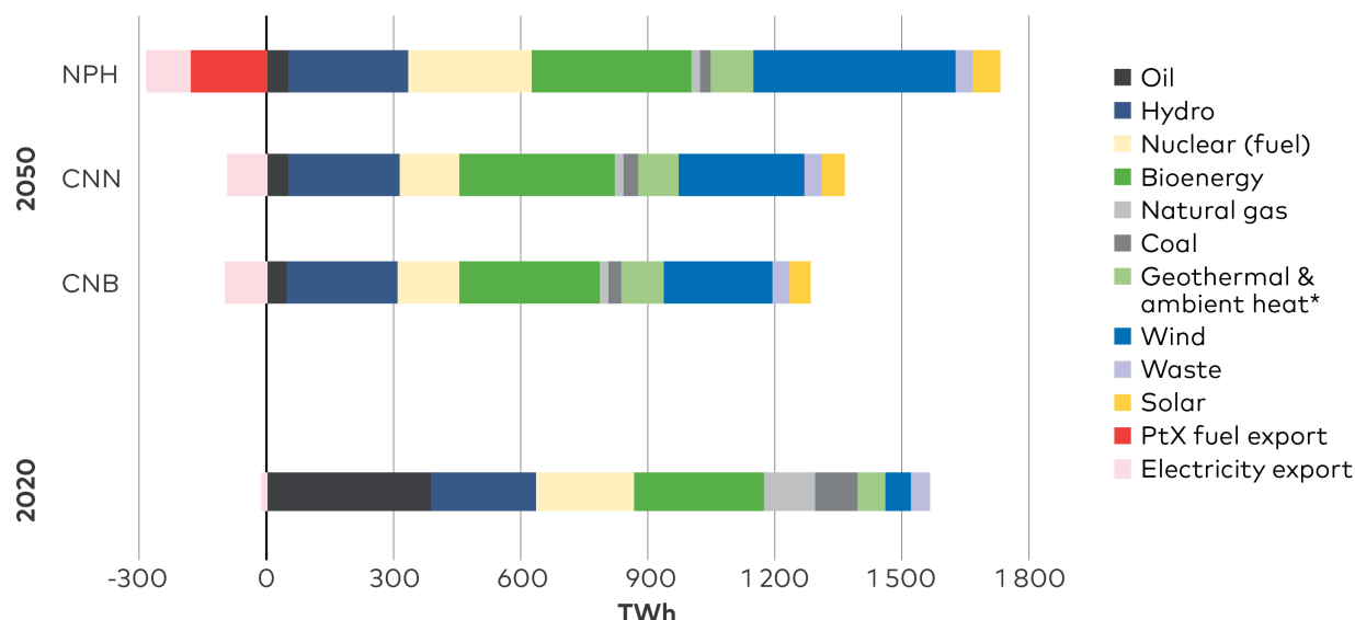
Figure 2.1. Total primary energy supply.
