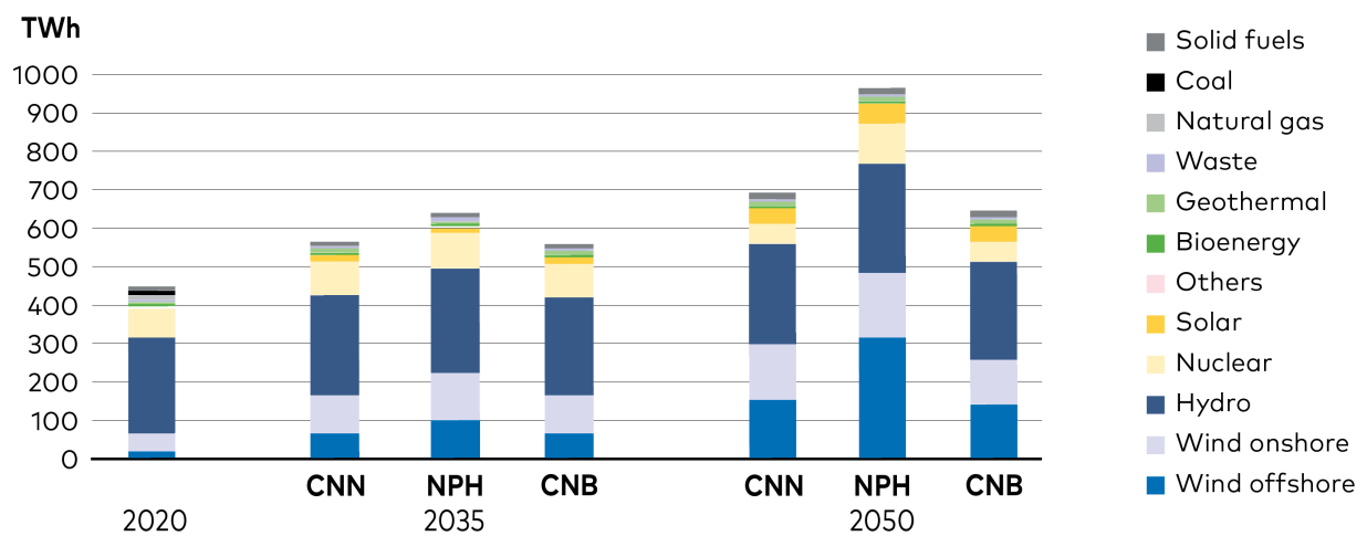
Figure 2.3. Nordic electricity generation.
