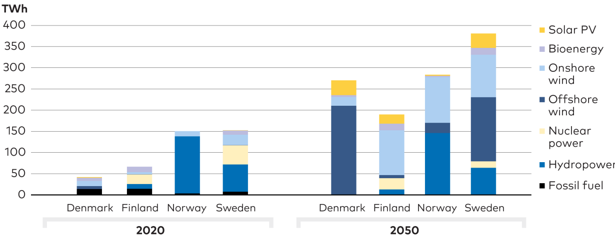
Figure 8.4. Total energy generation by source - HighPtX case. Total generation by energy source in the Nordic countries in 2020 and 2050 in the HighPtX case.
