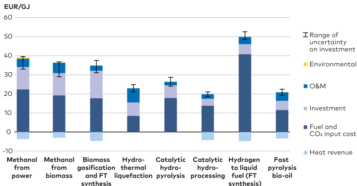
Figure 5.11. Levelized cost of fuel - 2030.
