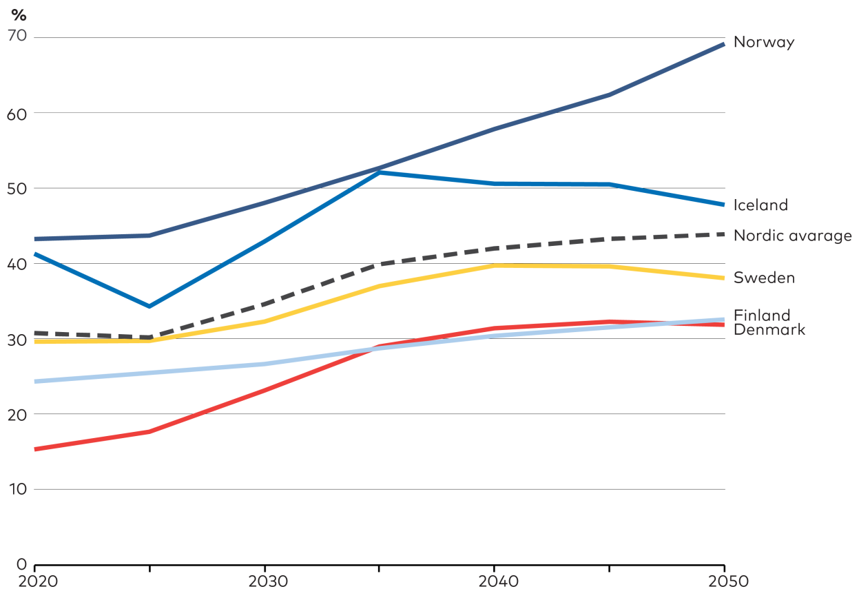
Figure 3.1. Final electricity demand as a share of total final energy demand – CNN scenario.
